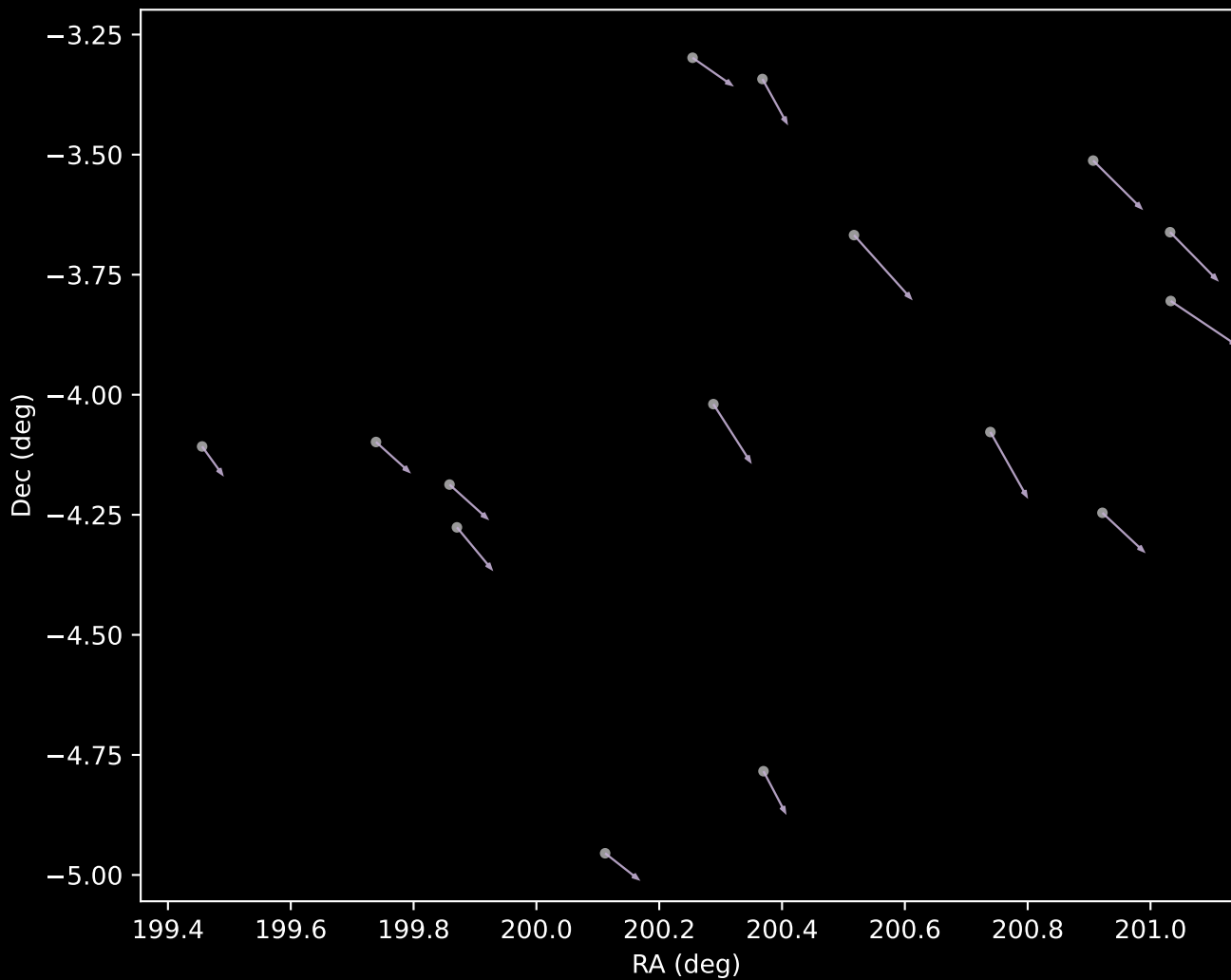
GALAH DR4 Cluster 9 Proper Motion Vectors (n=15)
