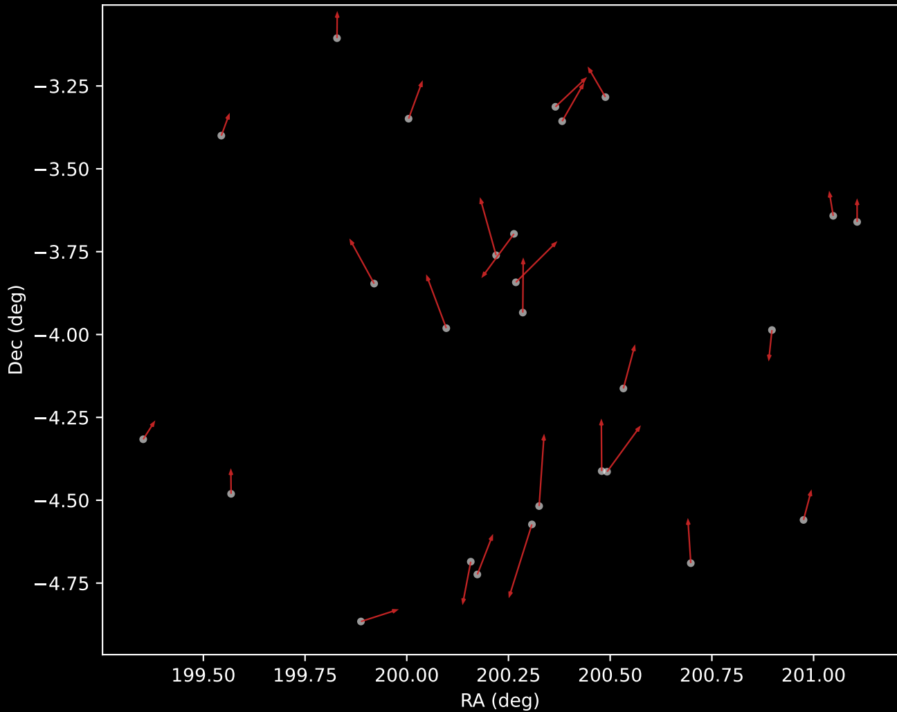
GALAH DR4 Cluster 6 Proper Motion Vectors (n=27)
