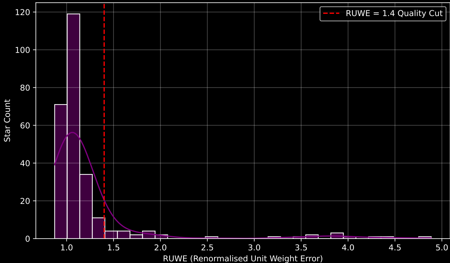
GALAH DR4 Field [9094] RUWE Distribution (n= 263)
