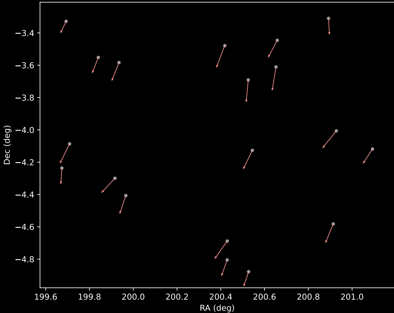
GALAH DR4 Cluster 7 Proper Motion Vectors (n=19)
