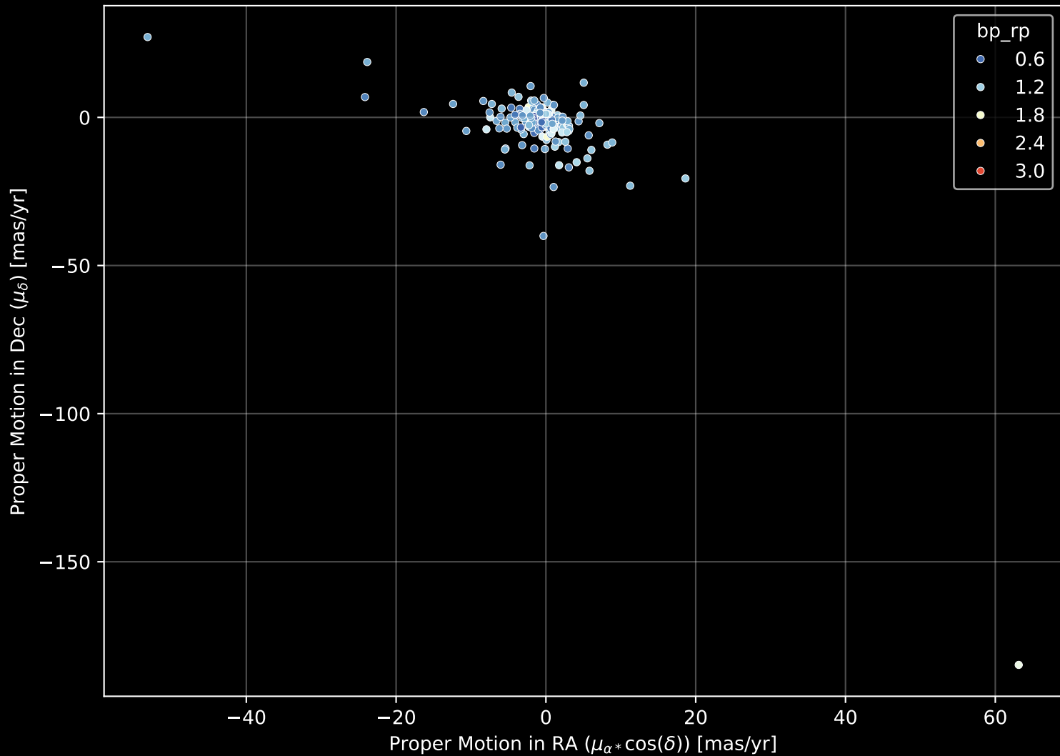
GALAH DR4 Field: [9094] Proper Motion Diagram (n= 270)
