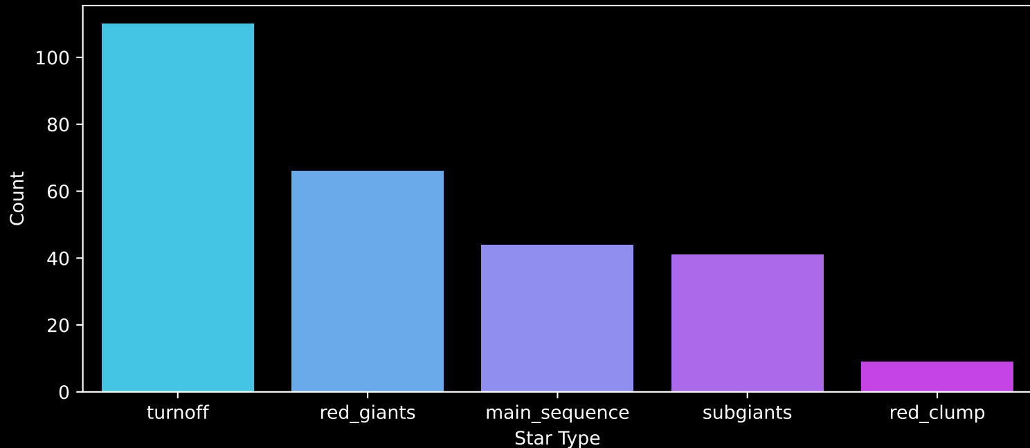
GALAH DR4 Field: [9094] Count plot of Star Type
