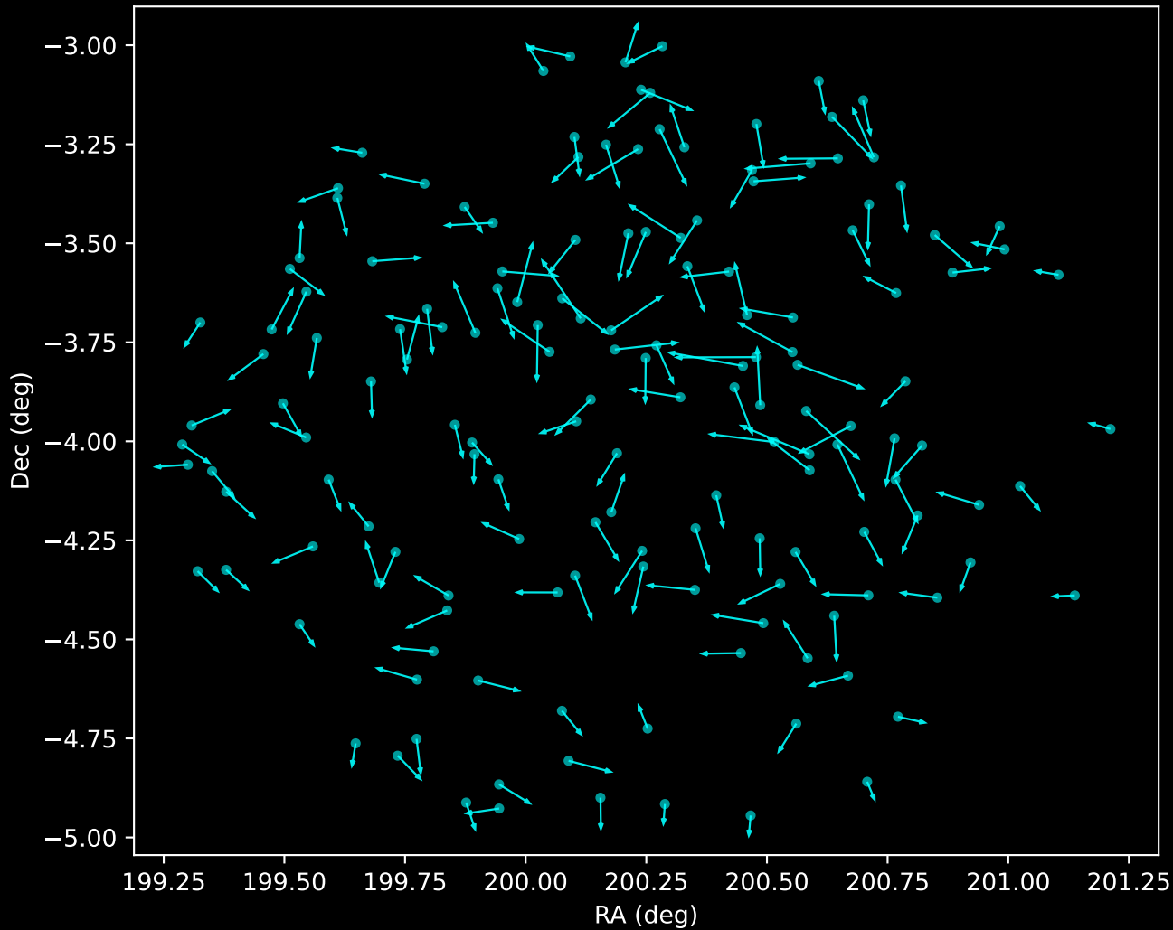
GALAH DR4 Noise Stream Proper Motion Vectors (n=156)
